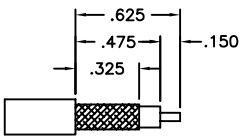
STRIPPING DIMENSIONS
